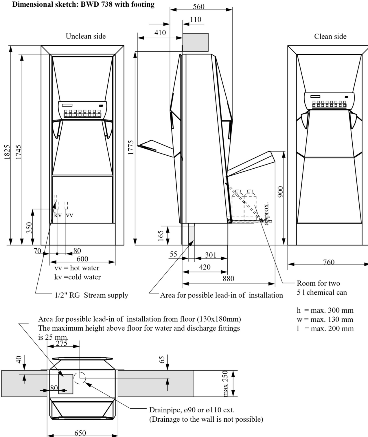
Dimensional sketch: BWD 738 with footing
