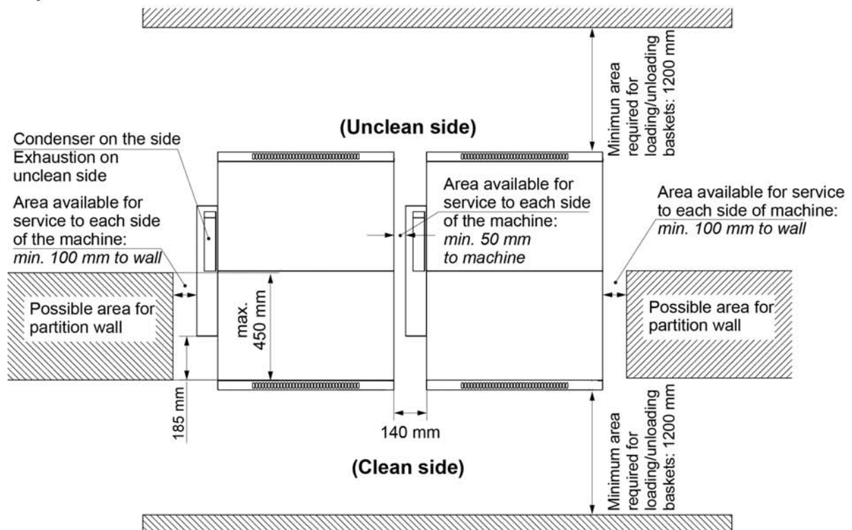
Top view
